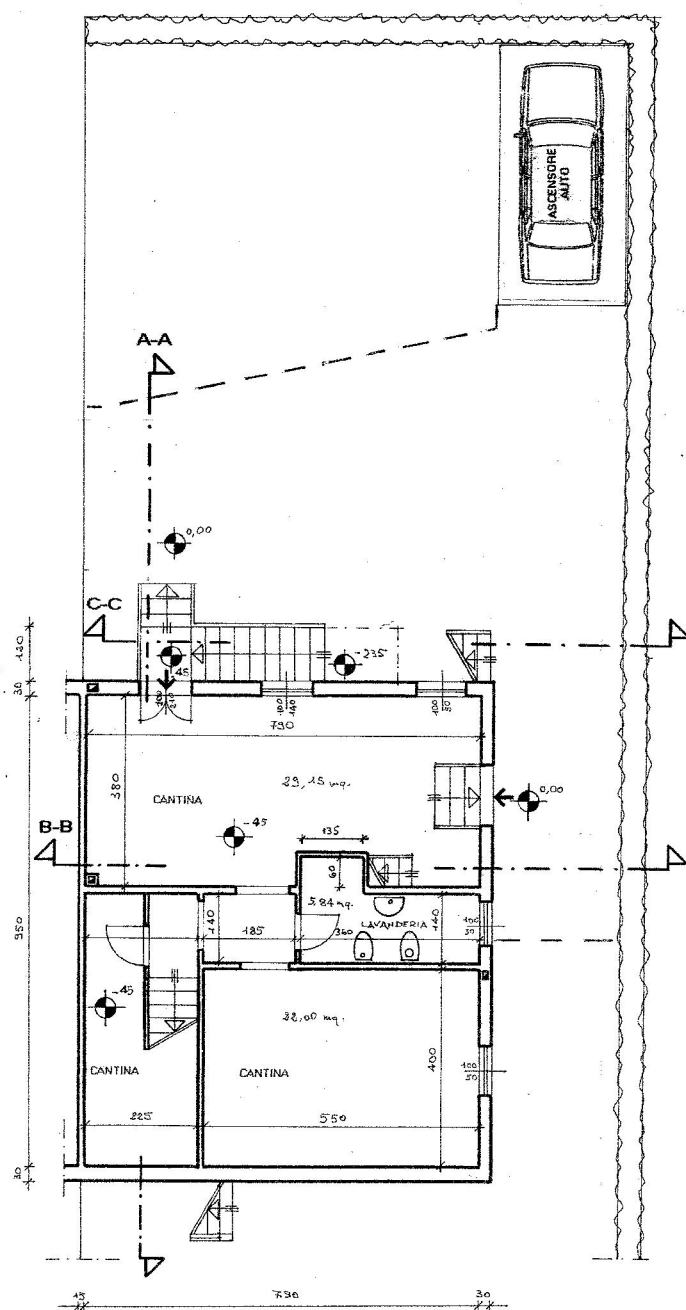
PIANO SEMINTERRATO
